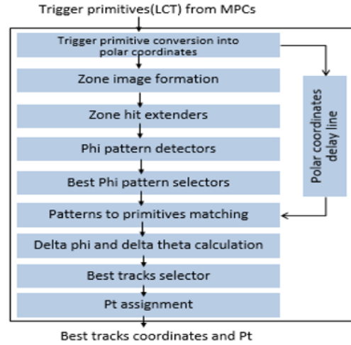
Figure 2. CSC track finder logic.
