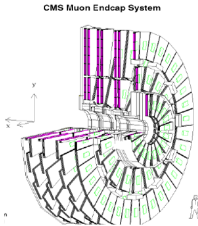
Figure 1. CMS Endcap Muon system.
